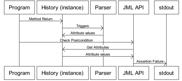
Figure 8: Sequence Diagram of postcondition assertion failure
